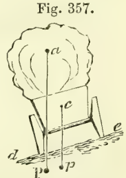
Fig. 357. Condition of Equilibrium.
